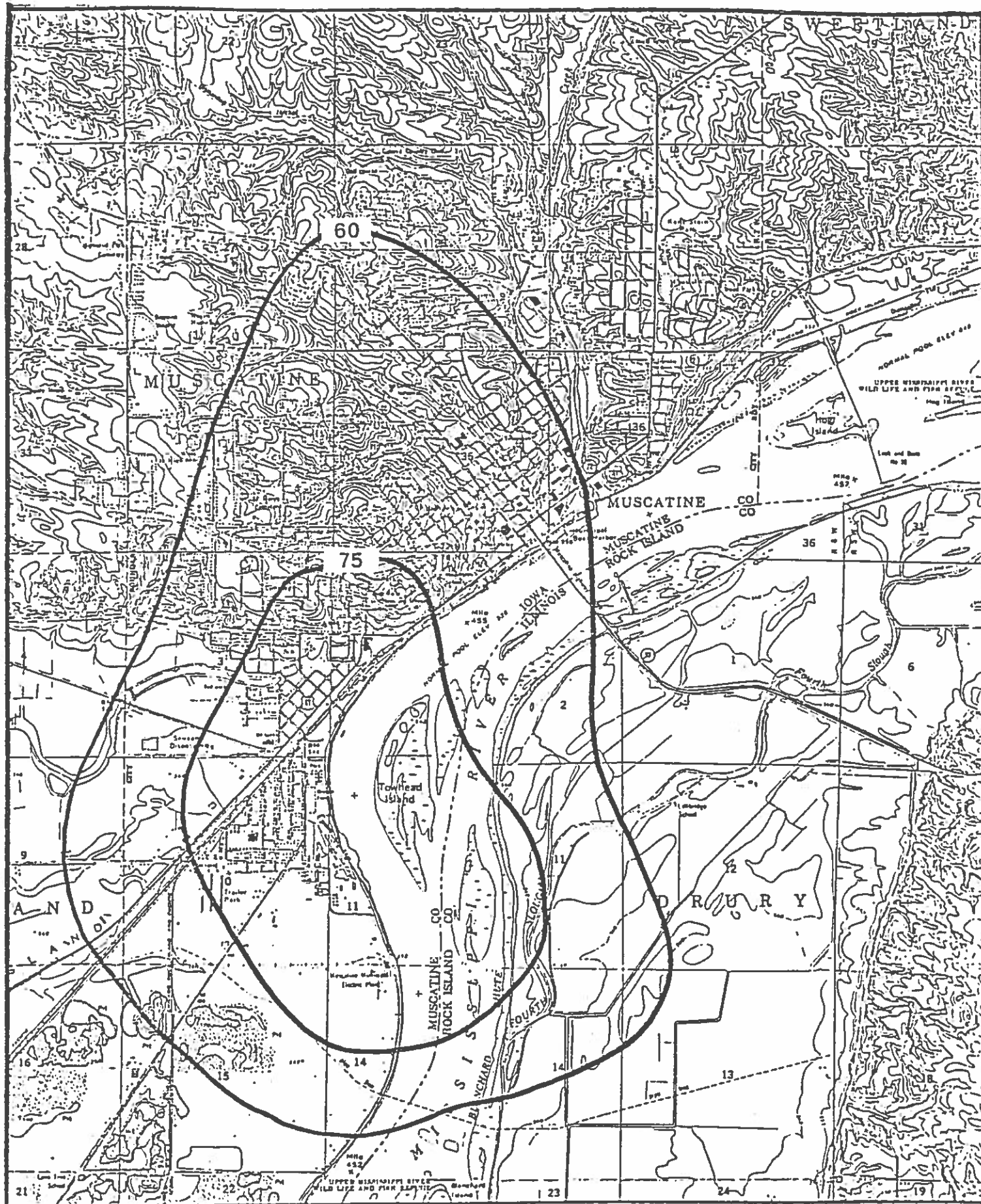
Figure 3-1 Suspended Particulate Isopleth Map for Muscatine (Values shown are geometric means in micrograms per cubic meter)
